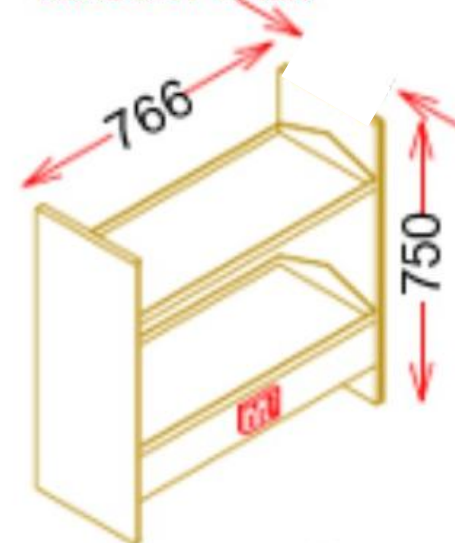
REAGENT RACK
